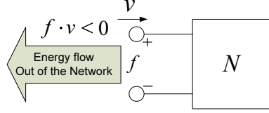
(b) Energy flow out of the network systems when f \cdot v < 0 .
