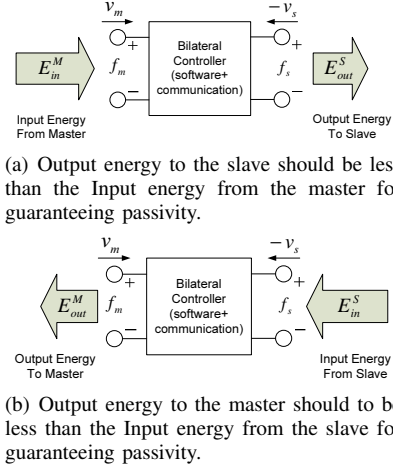
Fig. 6. In teleoperation systems with bilateral control law, the main source of the output energy at one port is the input energy at the other port, and the output energy should be less than the input energy.
