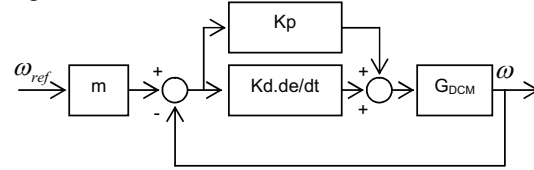
Fig. 4. Proposed control algorithm with PD control
